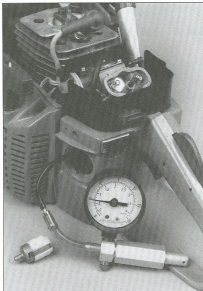
When pressure testing the fuel system, you need not wait for the inlet needle to pop off. You can open the inlet needle by cranking the engine or by tickling the metering diaphragm through the atmospheric vent hole. If the inlet needle re-seats below 10 psi, or does not re-seat, follow the procedures on p. 17 & 18.
