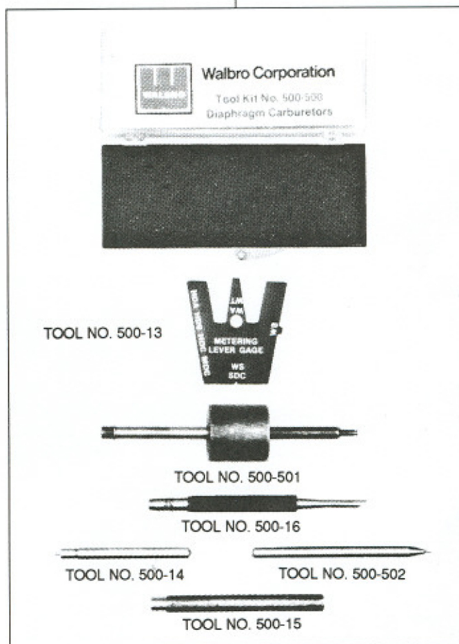
500-500 Tool Kit
