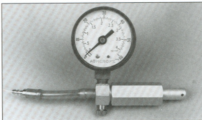
57-11 Pressure Tester
