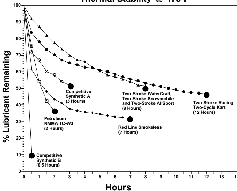
Thermal Stability @ 475°F
