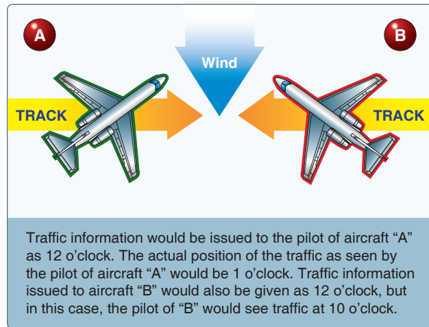
Figure 14-44. Traffic advisories.
