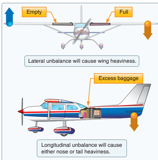
Figure 10-1. Lateral and longitudinal imbalance.
