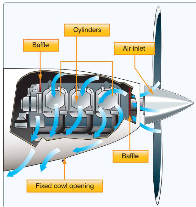
Figure 7-19. Outside air aids in cooling the engine.
