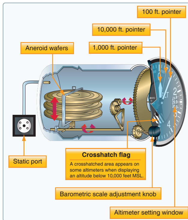
Figure 8-2. Altimeter.
